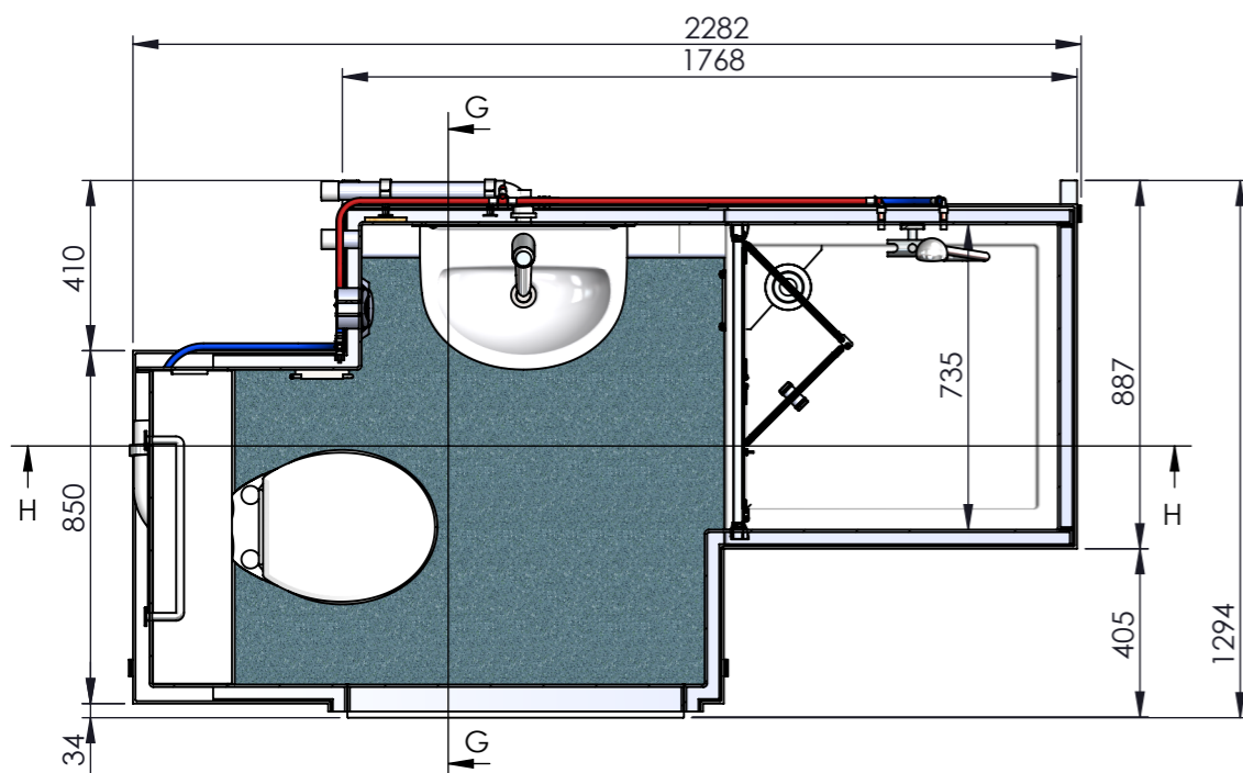
SECTION E-E
