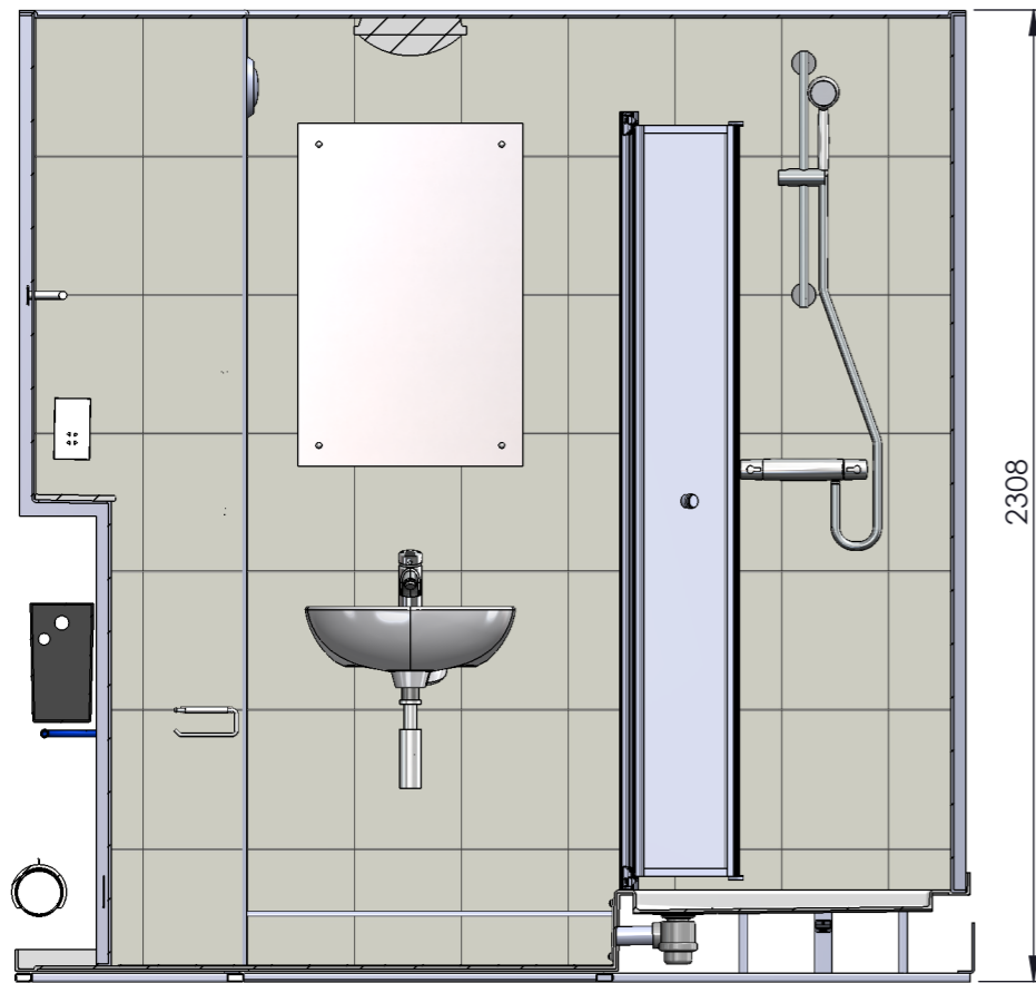
SECTION H-H
